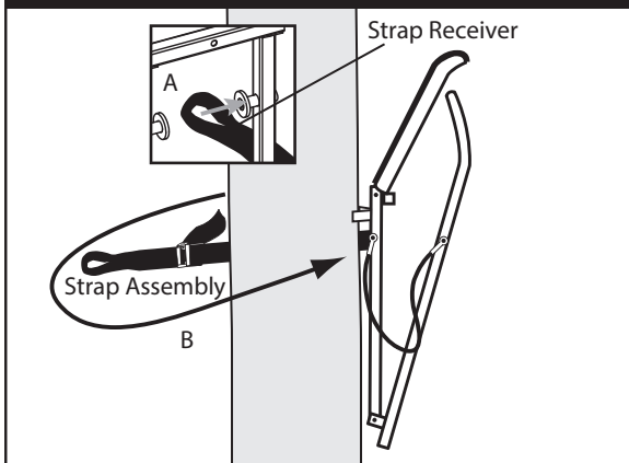
Fixed Position Install • FIGURE 3
