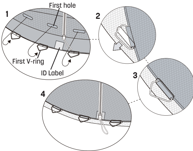
7 Enclosure Net (x1)
